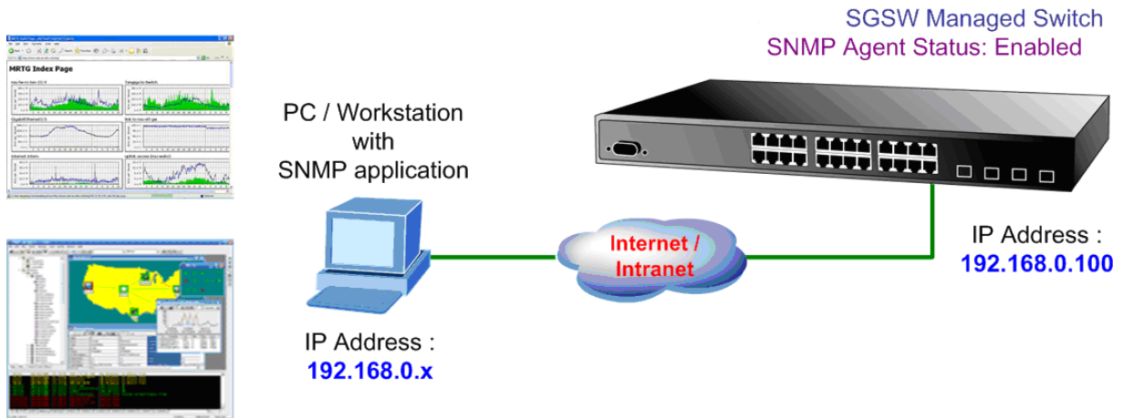
Figure 3-5 SNMP management
