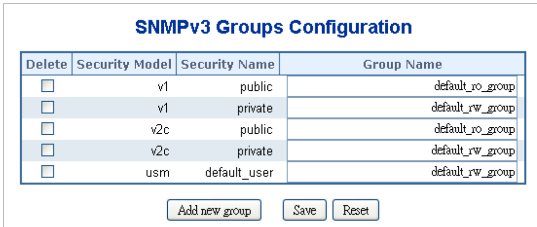
Figure 4-3-6 SNMPv3 Groups Configuration page screenshot
