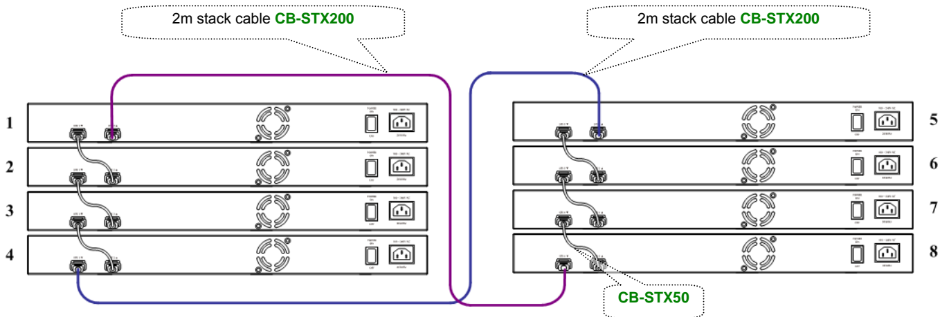
Figure 2-26 Separated Stack connection
