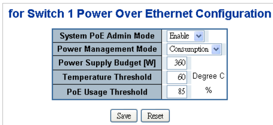
Figure 4-16-2 PoE Configuration screenshot
