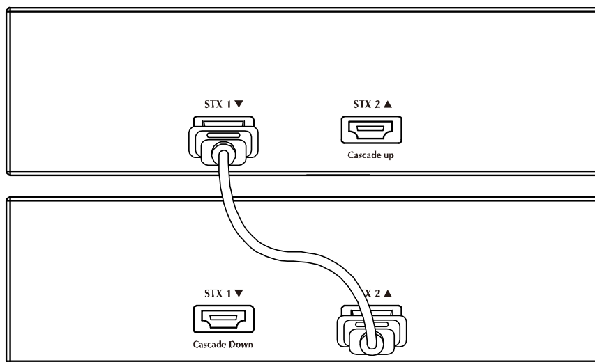
Figure 2-23 Stacking connection
