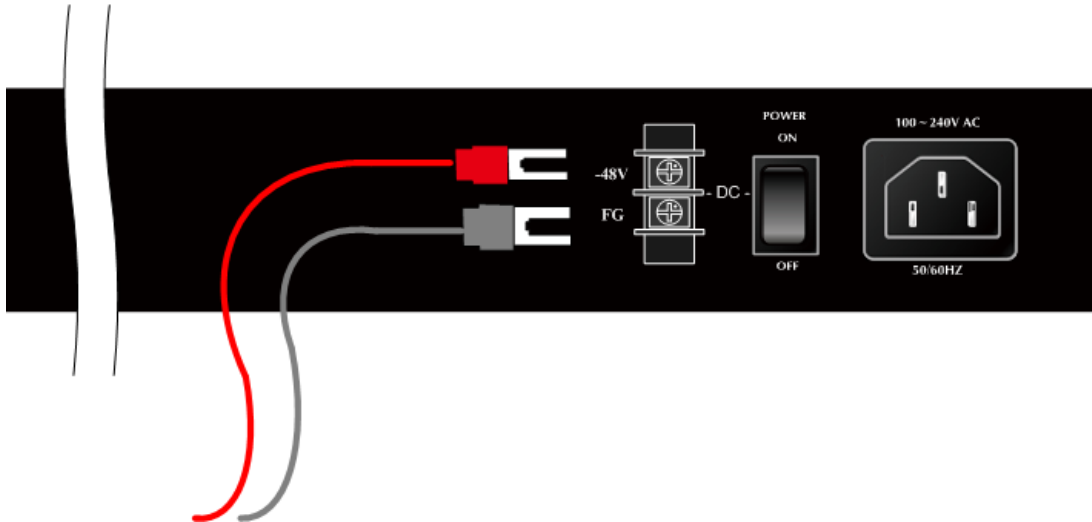
Figure 2-20 -48V DC connector
