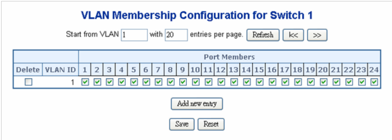
Figure 4-6-3 VLAN Membership Configuration page screenshot
