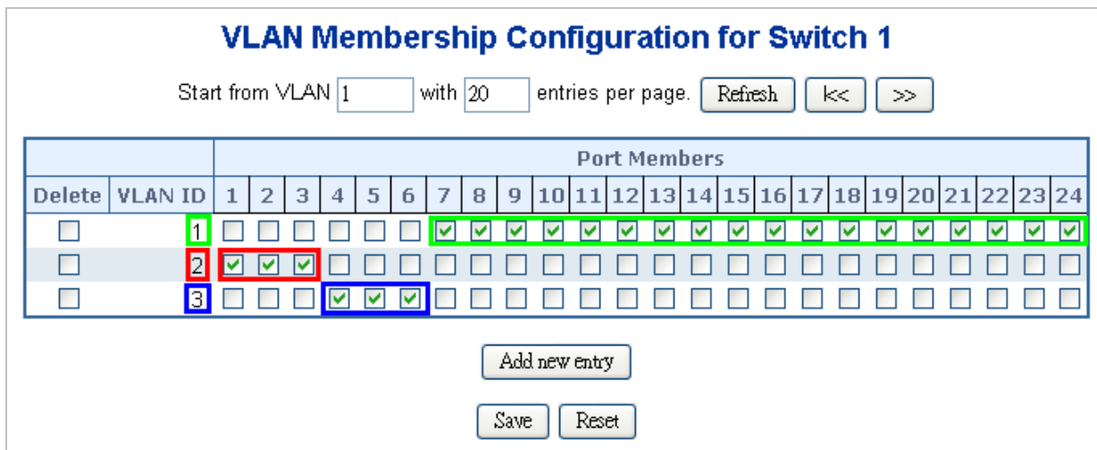
Figure 4-6-9 Add new VLAN group, assign VLAN members for VLAN 2 and VLAN 3 and remove specify ports from VLAN 1 member
