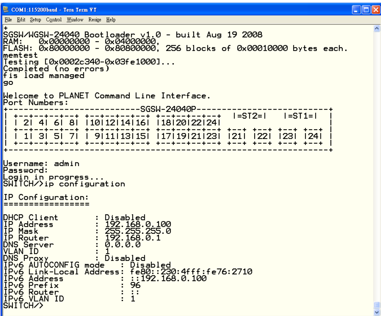
Figure 5-2 Show IP information screen
