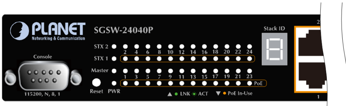
Figure 2-6 SGSW-24040P / SGSW-24040P4 LED panel
